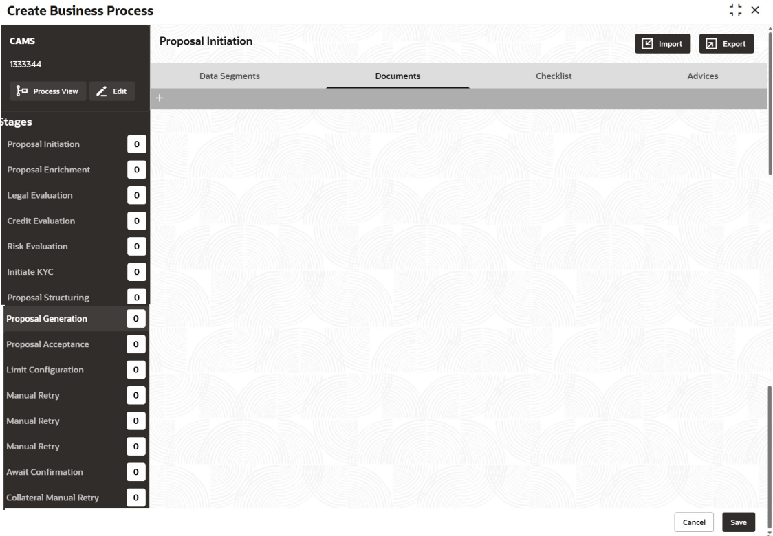
Figure 3-9 Documents Tab
